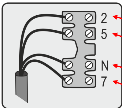
Black box from the FRONT of the electrobox
